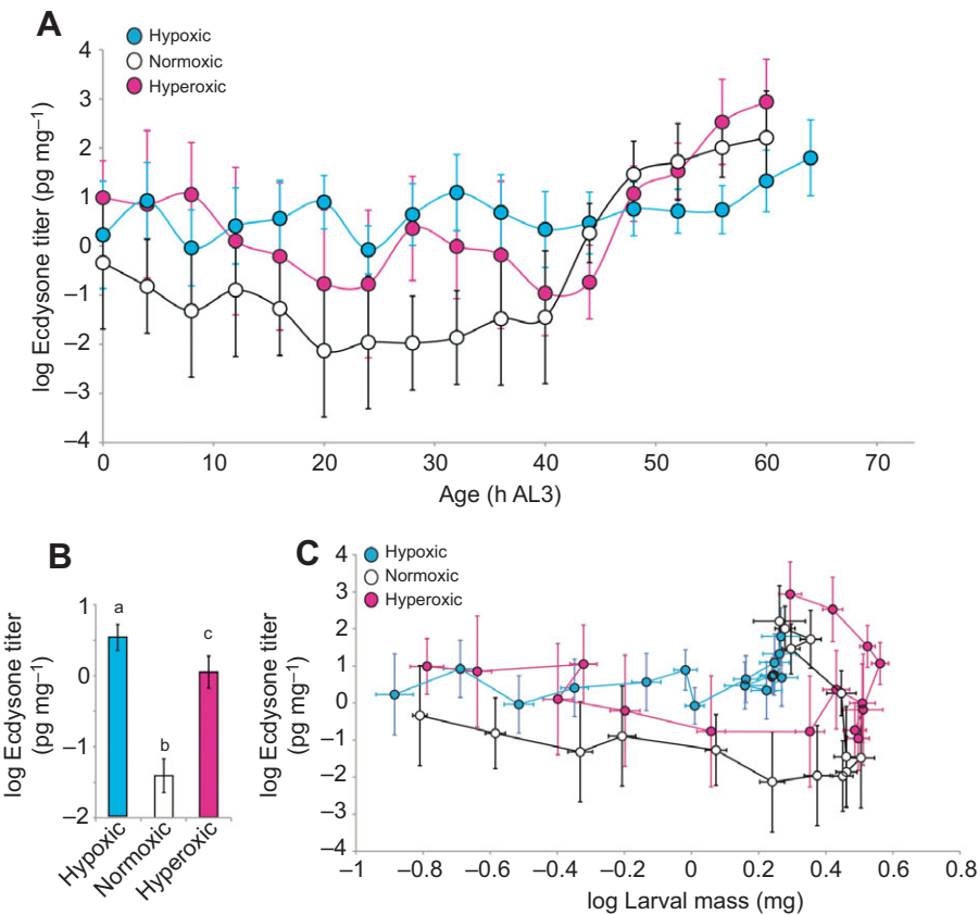
Fig. 5. Oxygen level affects the dynamics of the ecdysone titer. (A) Hormone titers of third instar larvae reared in hypoxic (cyan), normoxic (white), and hyperoxic (magenta) conditions as a function of time. (B) The mean ecdysone titer in larvae younger than 40 h AL3 is higher in hypoxic and hyperoxic conditions, controlling for larval age (ANOVA, P<0.001 ). Bars with different letters are significantly different (Bonferroni-corrected P<0.0167 ). (C) Hormone concentration as a function of mass. In hypoxic conditions, the ecdysone titer rises in smaller larvae, but the masses at which the ecdysone peak occurred were similar for normoxic and hyperoxic larvae. All error bars are 95% confidence intervals.
